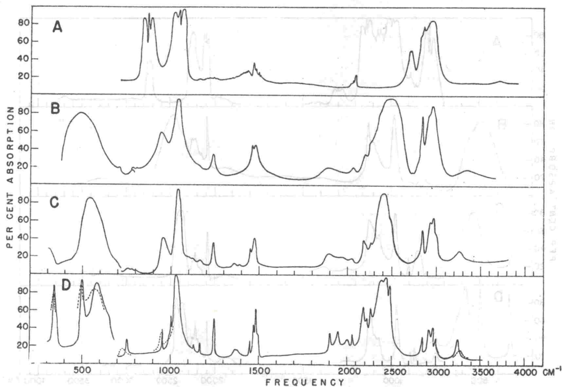
FIG. 2. Infrared absorption spectrum of \text{CH}_3\text{OD} . A—Vapor, 10-cm path-length, 80 mm Hg pressure, room temperature. B—Liquid, room temperature. C—Vitreous solid, -180^\circ\text{C} . D—Crystalline solid, -180^\circ\text{C} (full line) and -108^\circ\text{C} (broken line, shown only where the spectrum differs appreciably from that at -180^\circ\text{C} ).
